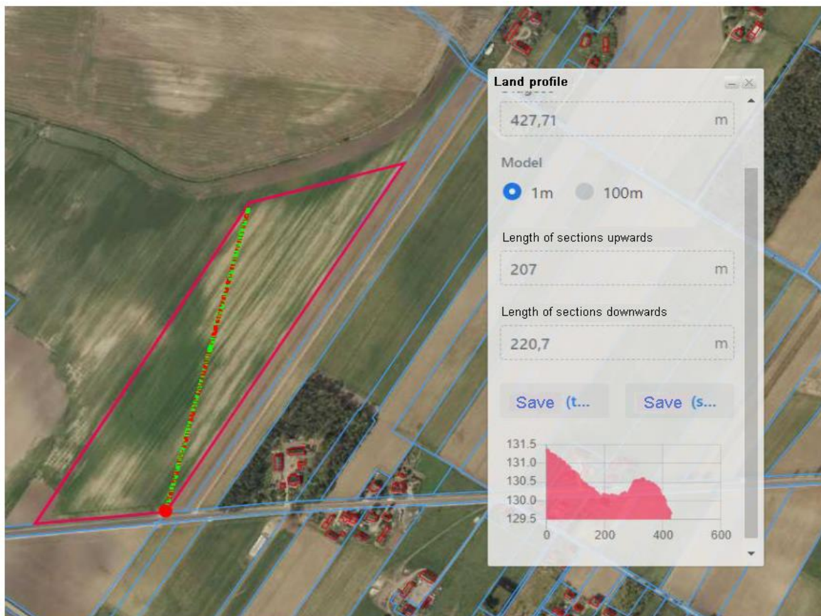
Fig. 4. Land profile of the project area for the photovoltaic farms
